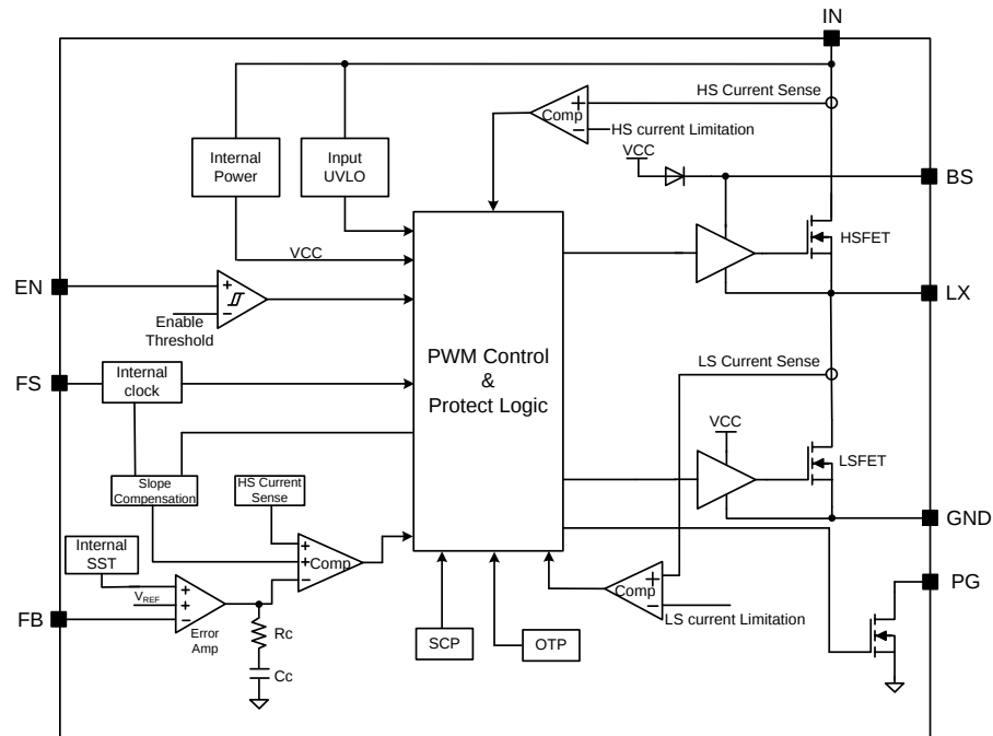
Figure3. Block diagram
