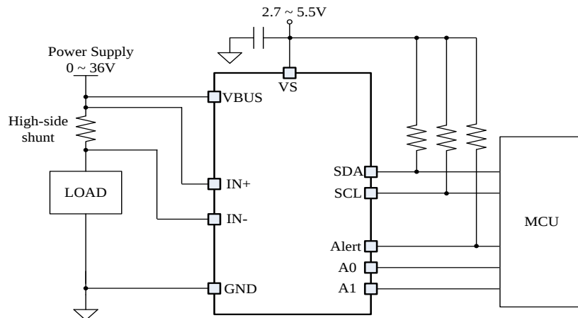
Figure 1. Typical Application
