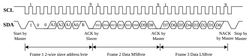
Figure 7. Timing Diagram for Read Word Format
