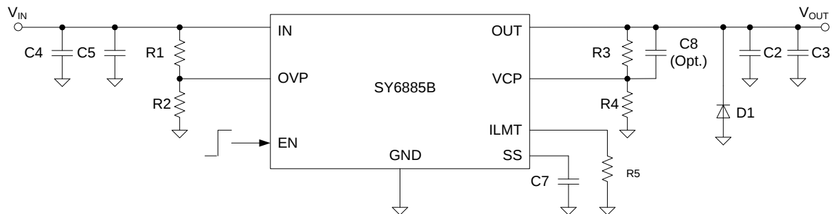
Figure 1. Schematic Diagram
