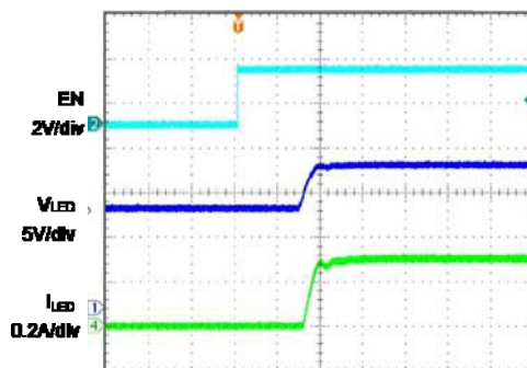
Startup from Enable
