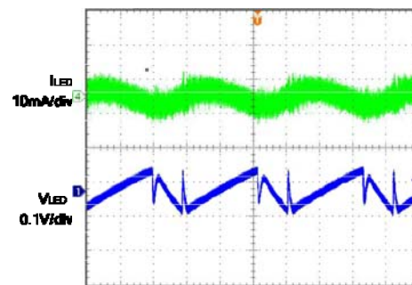
LED Current Ripple
