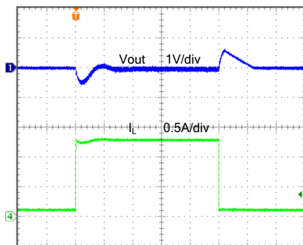
Load Transient V_{IN} = 5.0V, V_{OUT} = 12V, I_O = 0.1 \sim 1.3A
