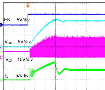
Startup from Enable V_{IN} = 5.0V, I_O = 1.0A
