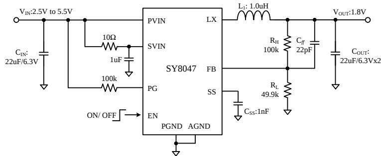
Figure 1. Schematic Diagram
