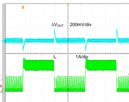
Load transient ( V_{IN}=24V , V_{OUT}=5V , I_{OUT}=0.2A \rightarrow 2A )
