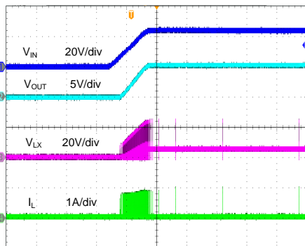
Startup from V_{IN} ( V_{IN}=24V , V_{OUT}=5V , I_{OUT}=0A )
