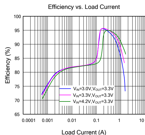
Figure 2. Efficiency Figure
