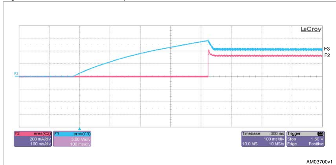
Figure 3. VIPER22A-E startup
