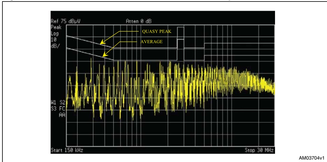
Figure 7. Conducted emissions at 230 VAC 50 Hz - line 1 peak detector
