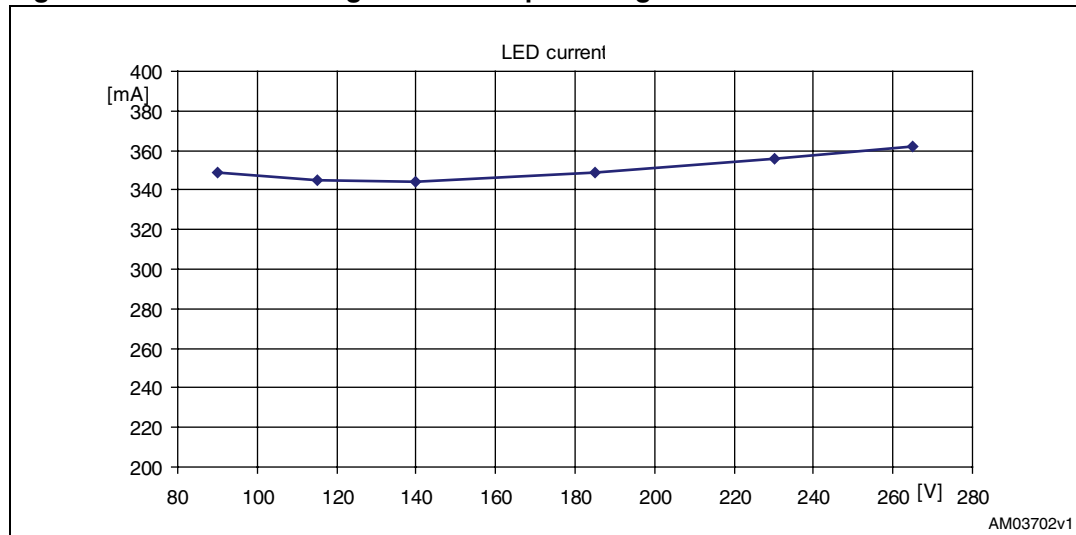
Figure 5. LED current regulation vs. input voltage
