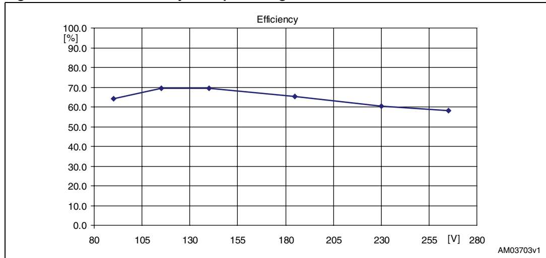
Figure 6. Board efficiency vs. input voltage
