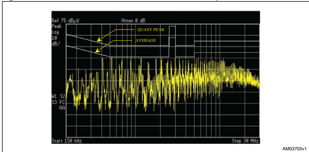
Figure 8. Conducted emissions at 230 VAC 50 Hz - line 2 peak detector
