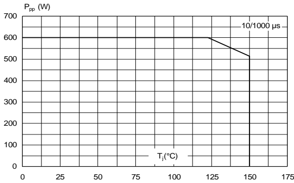
Figure 3: Peak power dissipation versus initial junction temperature (typical values)
