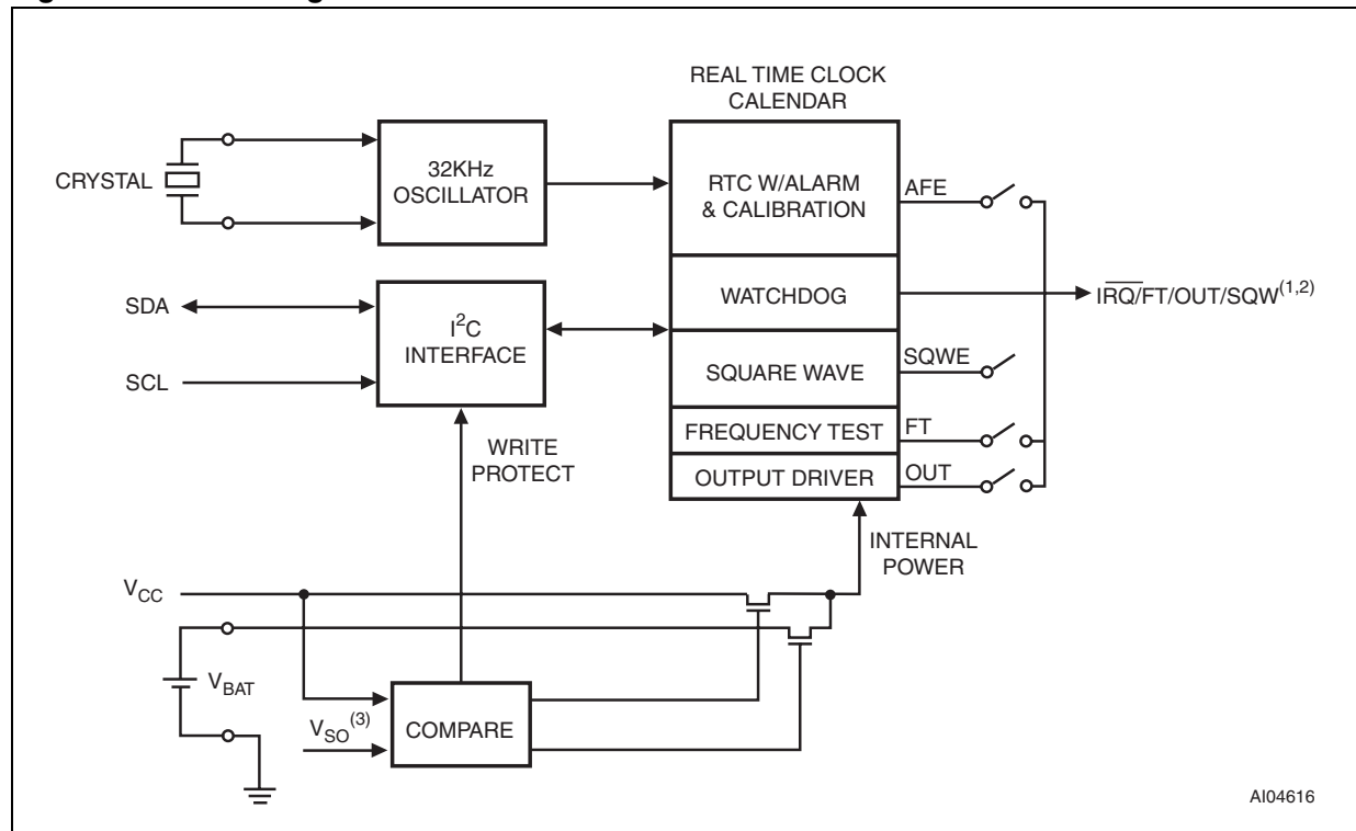
Figure 3. Block diagram
