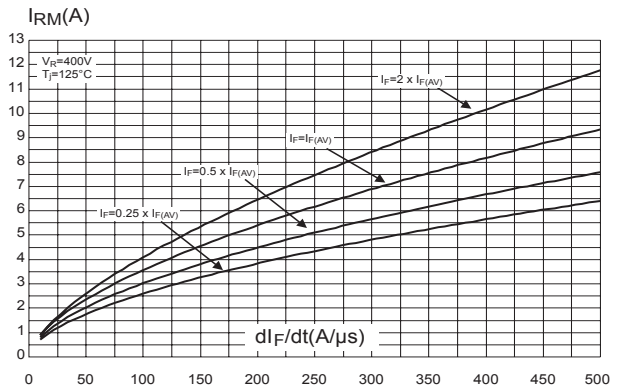
Figure 4. Peak reverse recovery current versus di/dt (typical values)
