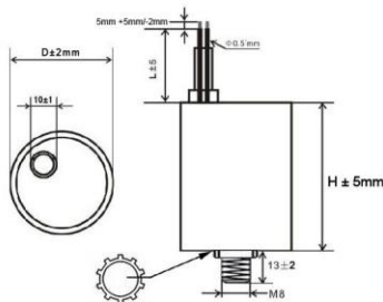
TS11-19 (only for D:30mm)
