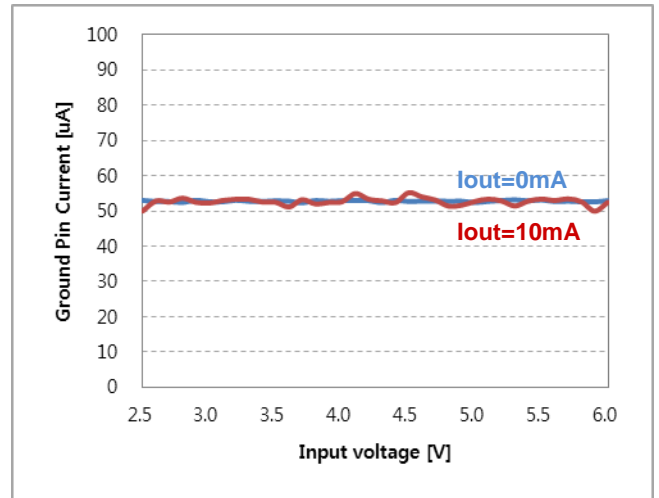
Ground Current @ I_{out}=0A / 10mA ( C_{in}=10\mu F , C_{out}=10\mu F , R_2=36K\Omega , R_1=35K\Omega )
