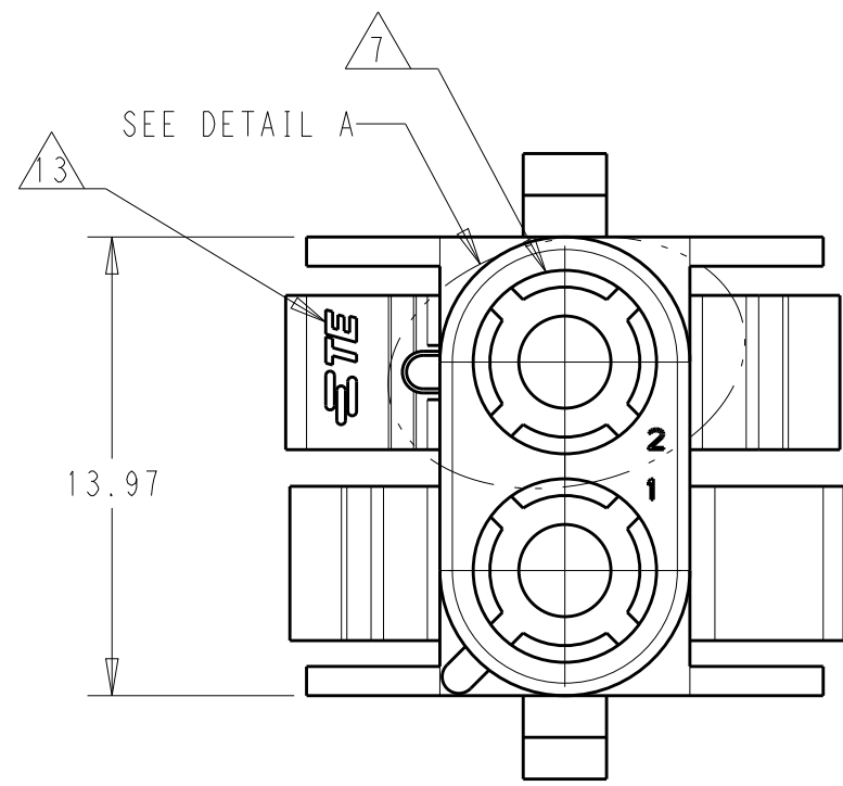
CONSTRUCTION OPTION 1
