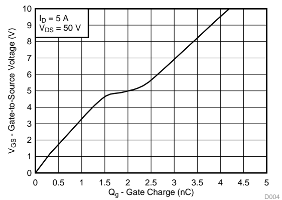
Gate Charge
