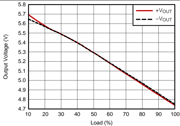
Figure 7. Load Regulation
