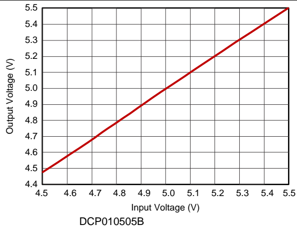
Figure 2. Line Regulation
