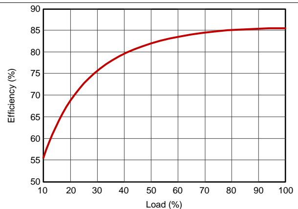
Figure 10. Efficiency vs Load
