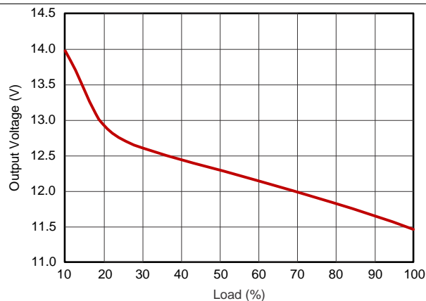
Figure 9. Load Regulation
