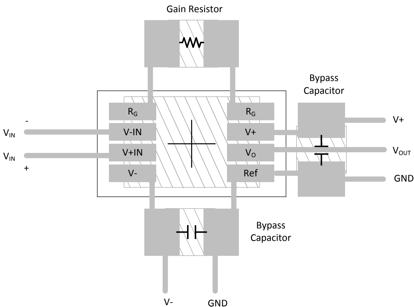
Figure 36. Layout Recommendation
