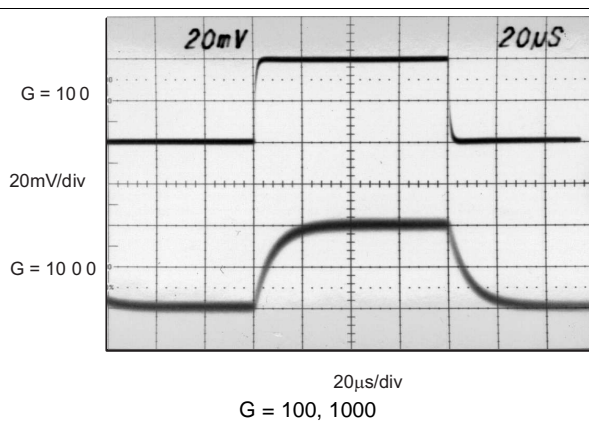
Figure 28. Small Signal
