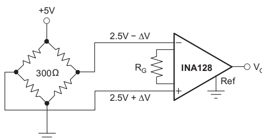
Figure 31. Bridge Amplifier
