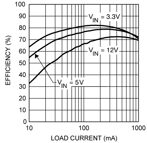
Figure 22. Efficiency vs Load Current - L1 = 10 µH V OUT = 1.5 V
