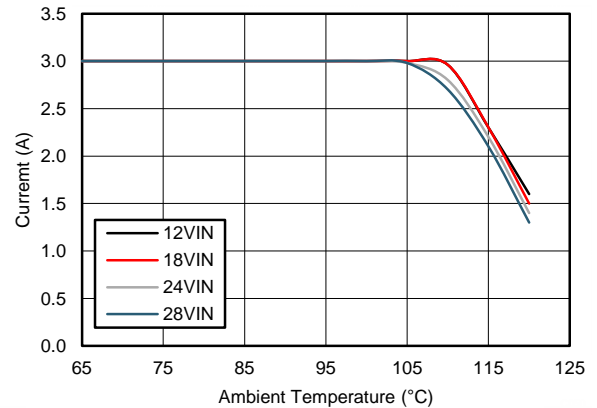
Figure 72. Derating Curve
