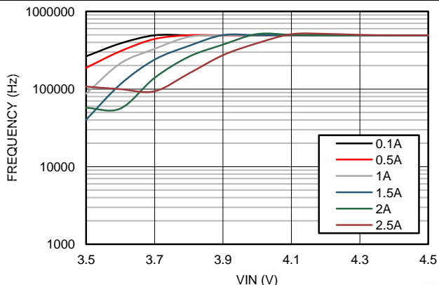
V_{OUT} = 3.3\text{ V} F_S = 500\text{ kHz}
