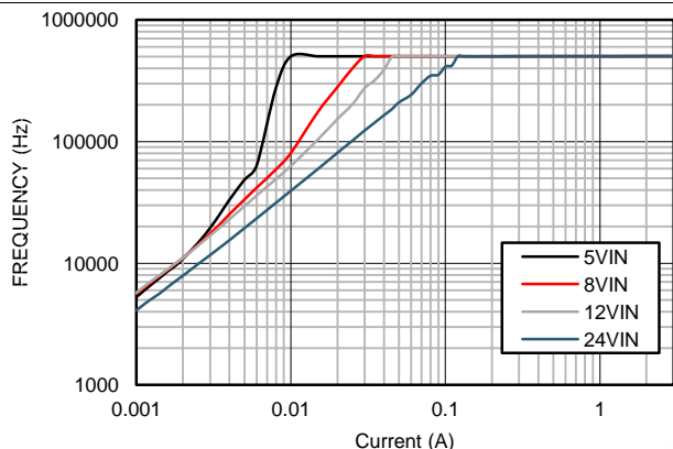
V_{OUT} = 3.3\text{ V} F_S = 500\text{ kHz}
