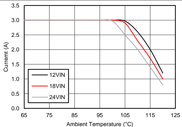
V_{OUT} = 3.3\text{ V} F_S = 500\text{ kHz} \theta_{JA} = 20^\circ\text{C/W}
