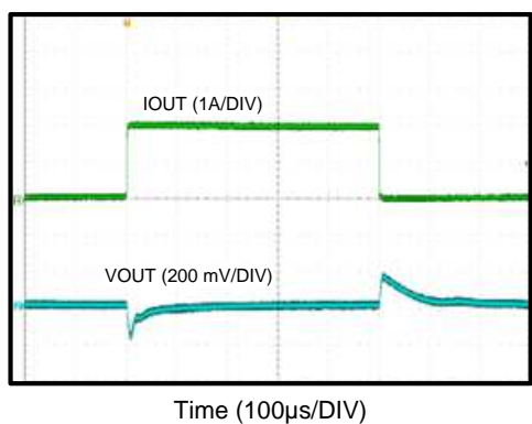
V_{OUT} = 3.3\text{ V} F_S = 500\text{ kHz}
