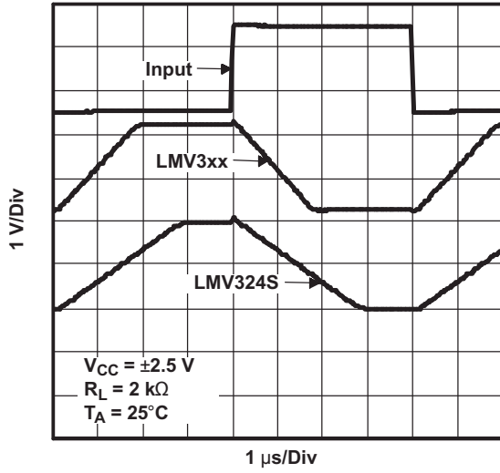
Figure 33. Inverting Large-Signal Pulse Response
