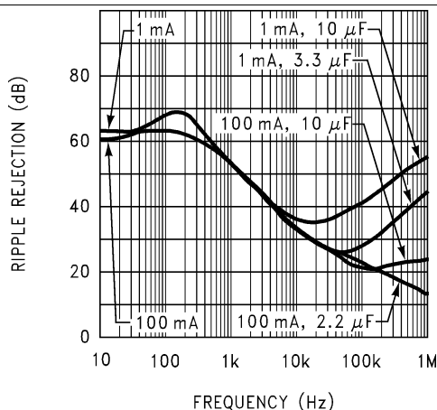
Figure 24. Ripple Rejection
