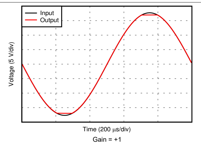
Figure 6-30. No Phase Reversal
