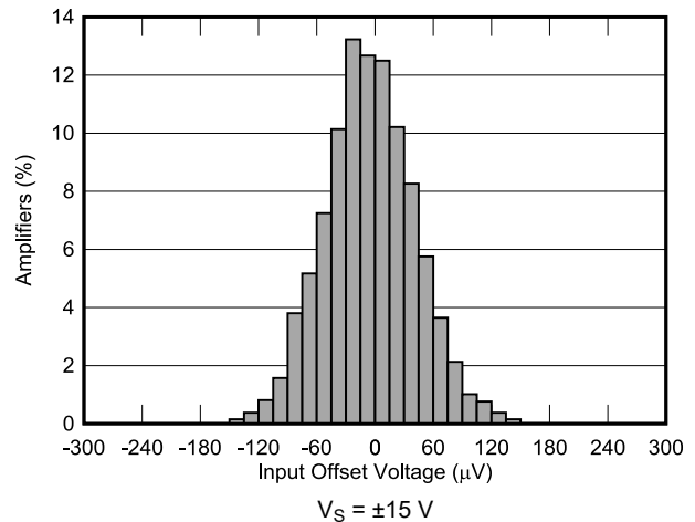
Figure 6-6. Offset Voltage Production Distribution
