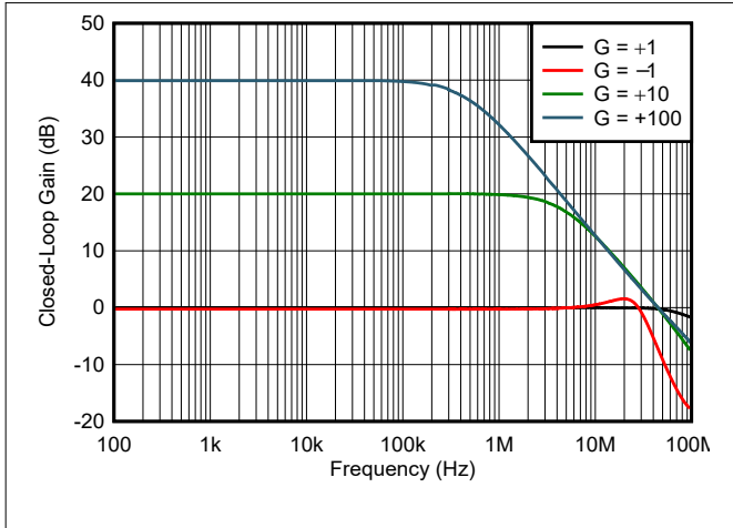
Figure 6-25. Closed-Loop Gain vs Frequency
