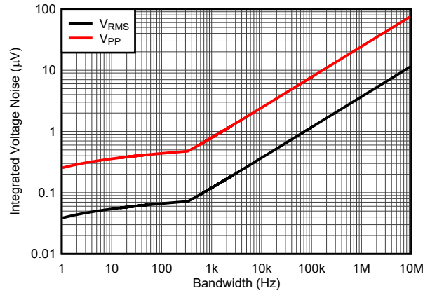
Figure 6-2. Integrated Input Voltage Noise vs Bandwidth
