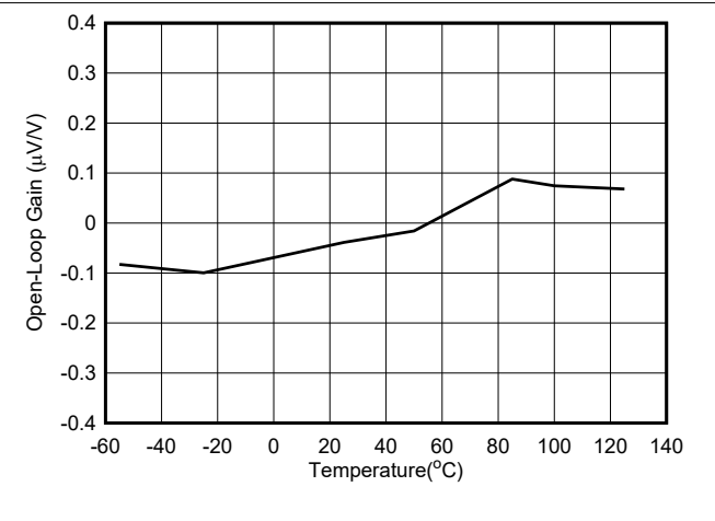
Figure 6-26. Open-Loop Gain vs Temperature
