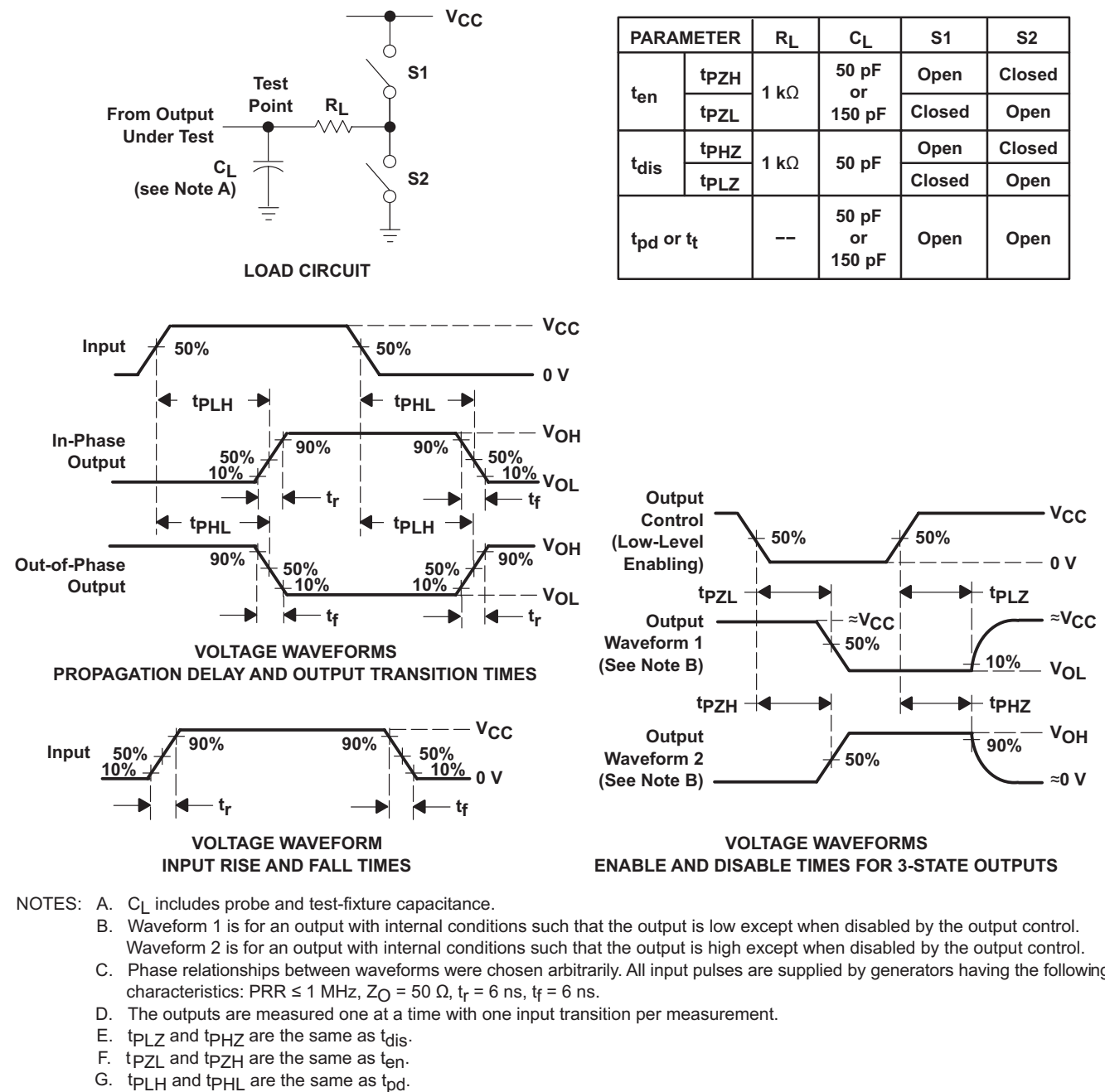
Figure 2. Load Circuit and Voltage Waveforms
