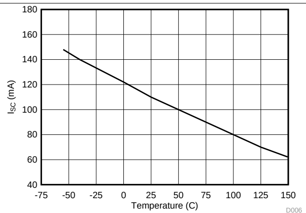
Figure 6. Reference Short Circuit Current vs Temperature for V_{IN} = 15\text{ V}
