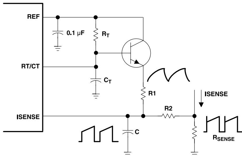
Figure 12. Slope Compensation
