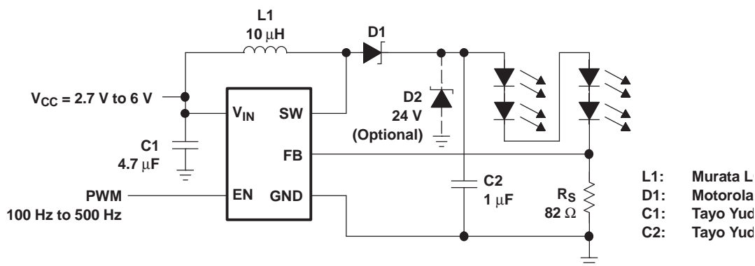
Figure 21. White LED Supply With Adjustable Brightness Control Using a PWM Signal on the Enable Pin, Efficiency Approximately Equals 86% at V_{IN} = 3 V, I_{LED} = 15 mA
