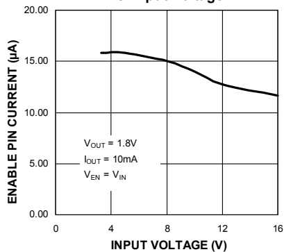
Enable Pin Current vs. Input Voltage
