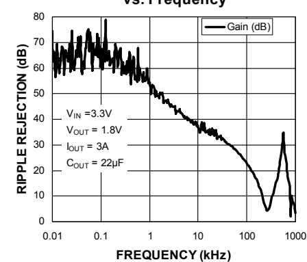
Ripple Rejection ( I_{OUT} = 3A ) vs. Frequency
