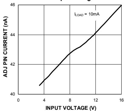
Adjust Pin Current vs. Input Voltage
