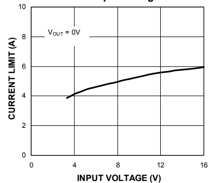
Short-Circuit Current vs. Input Voltage
