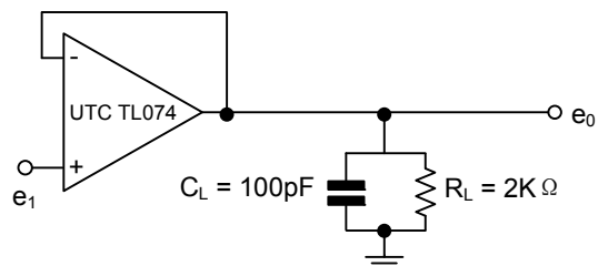
Figure 1. Voltage Follow
