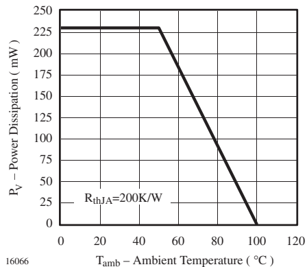
Figure 3. Power Dissipation vs. Ambient Temperature
