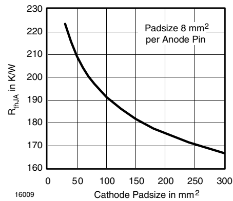
Figure 14. Thermal Resistance Junction Ambient vs. Cathode Pads Size
