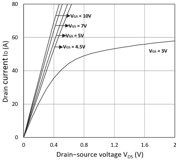
Figure 1. Output Characteristics
