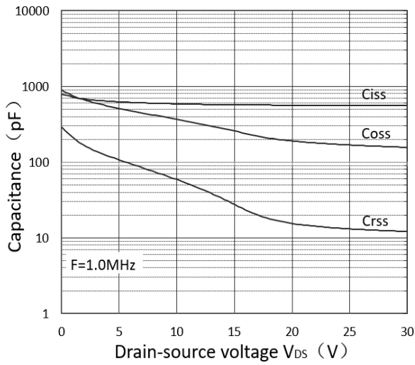
Figure 7. Capacitance Characteristics
