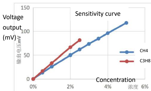
Fig3. Sensitivity Curve
