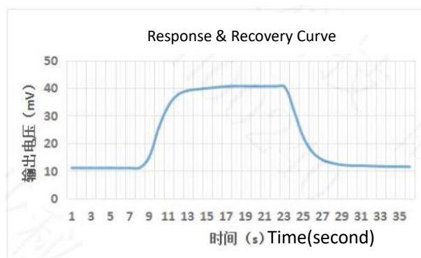
Fig4. Response and recovery
