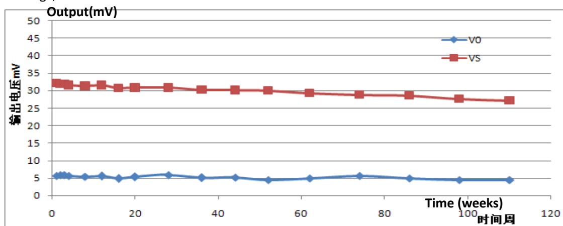
Fig11. Sensitivity fluctuation
