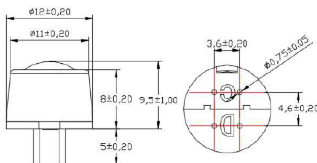
Fig1.Sensor Structure
