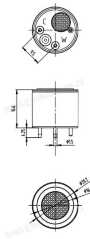
Figure 1: Sensor structure
