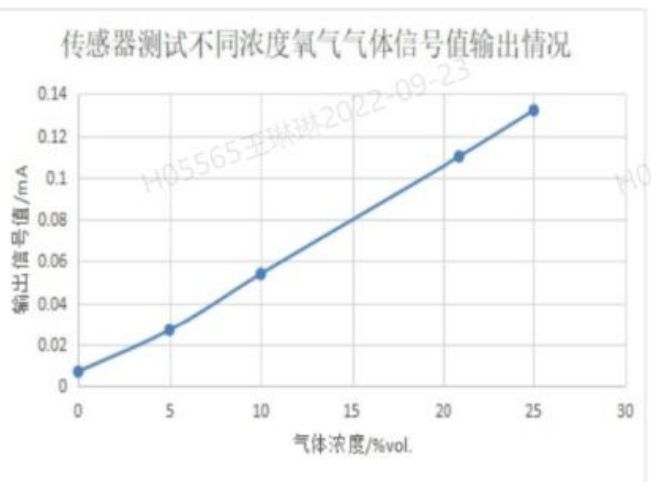
Figure 4: Sensor Linear Curve
