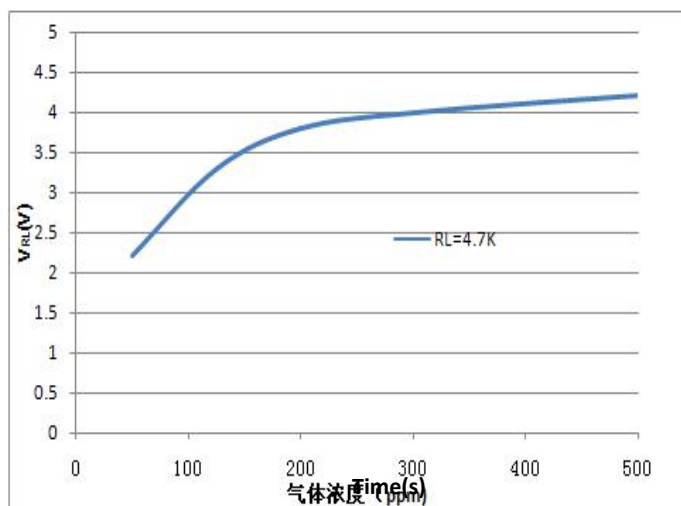
Fig5. Sensitivity Curve
