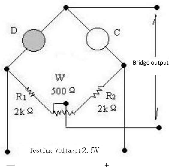
Pic 2: Basic Testing Circuit
