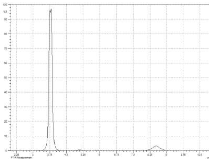
3.8um narrow band filter spectral curve
