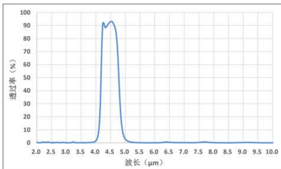
4.48μm narrow band filter spectral curve
