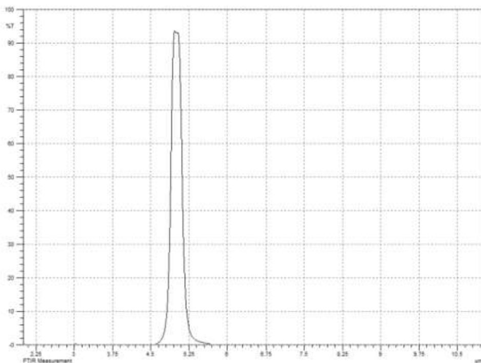
5.0μm narrow band filter spectral curve
