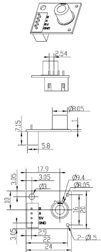
Picture 1:Module structure diagram
