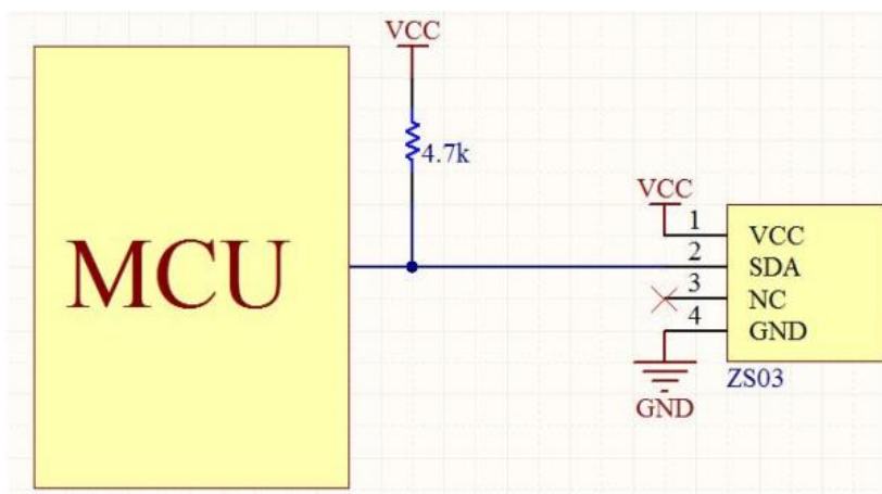
Fig3 Application circuit
