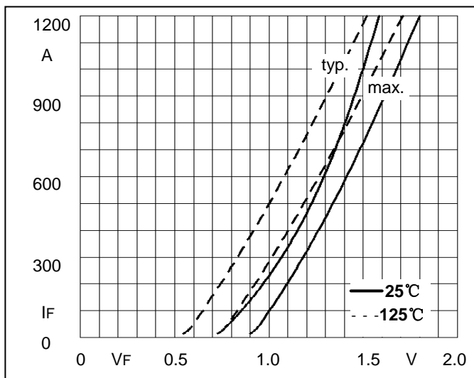
Fig5. Forward Characteristics
