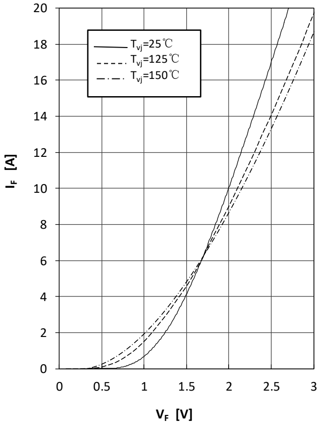
Fig13.Diode-brake-chopper Foward Characteristics
