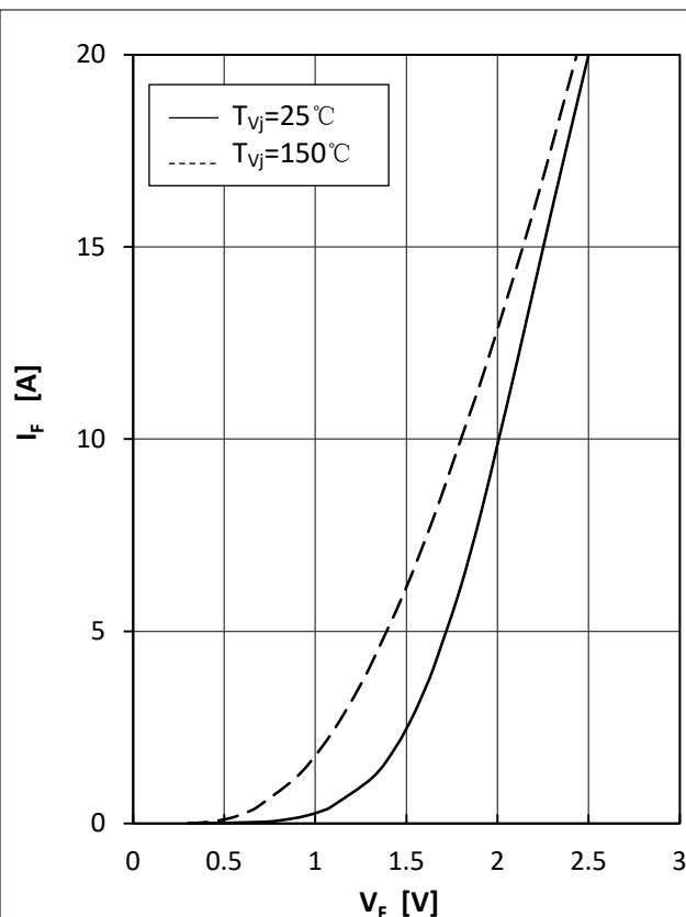
Fig13.Diode-brake-chopper Forward Characteristics
