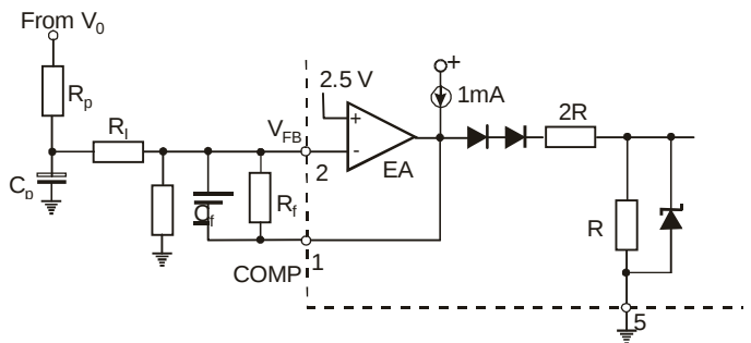
Figure 5. Latched Shutdown
