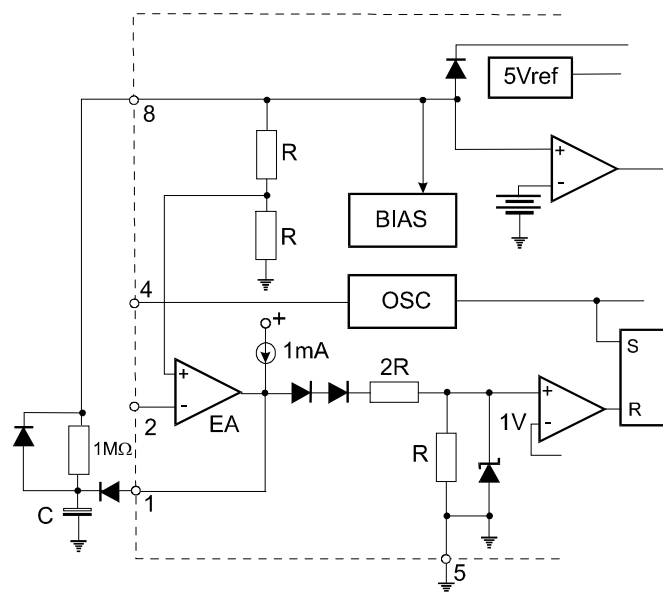
Figure 8. Soft-Start Circuit
