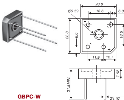
GBPC-W
