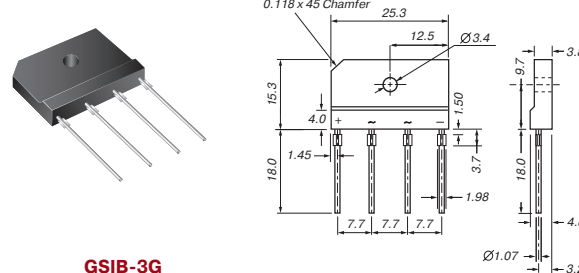
GSIB-3G
