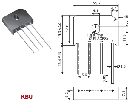
KBU
